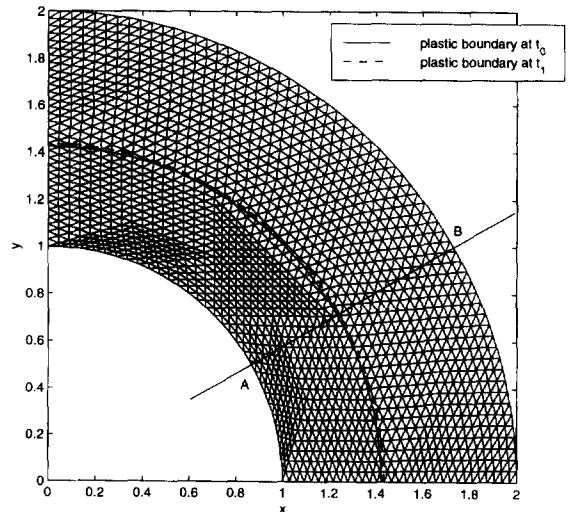
Fig. 4. Uniform mesh after 4 red-refinements in Example 8.1.
