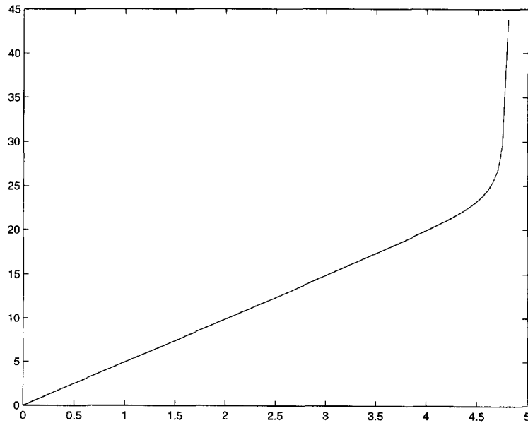
Fig. 13. \int_{\Gamma} u_2 ds versus t in Example 8.2.
