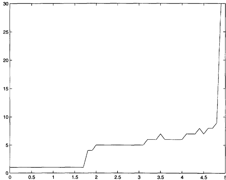
Fig. 11. Number of Newton iterates versus t , 0 \leq t \leq 5 in Example 8.2.
