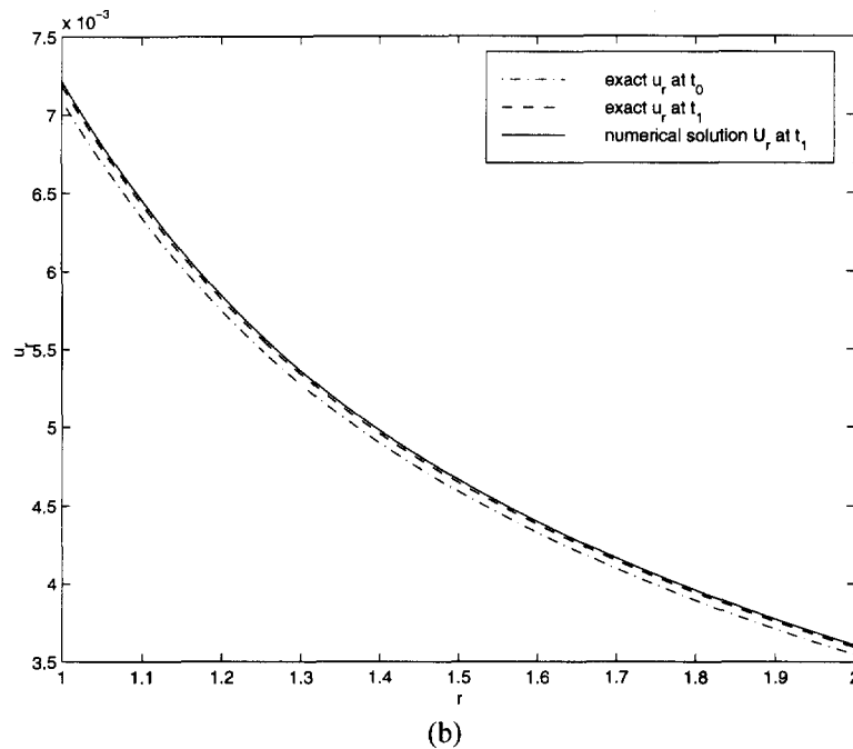
Fig. 6. Exact and discrete solution for the mesh shown in Fig. 7 along A–B in Example 8.1.
