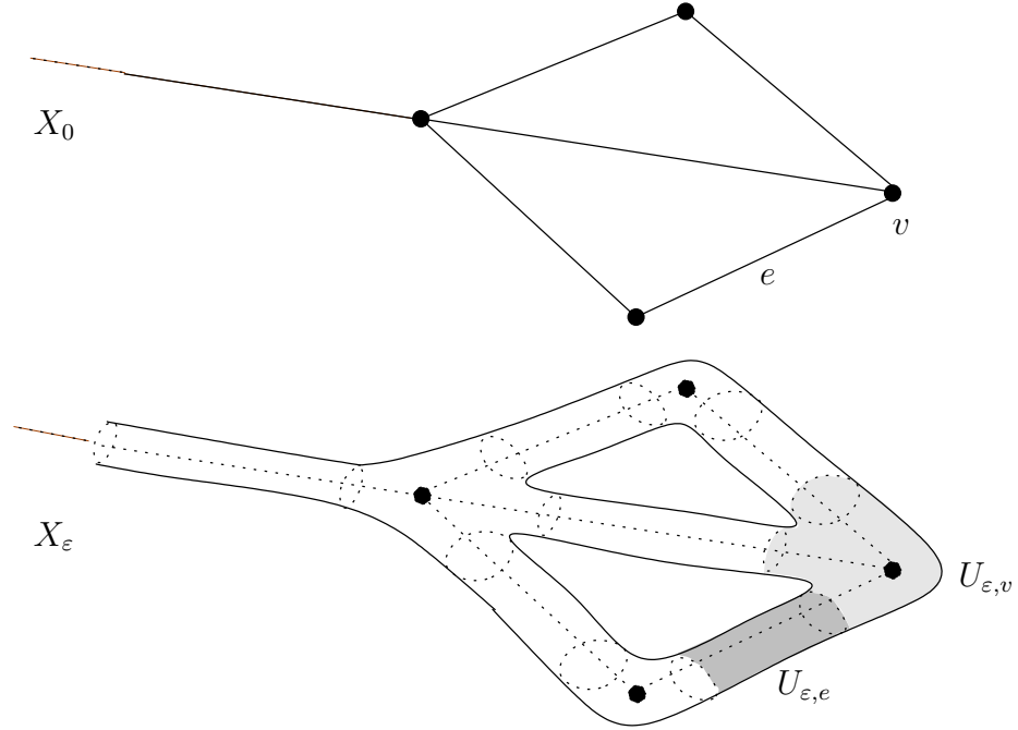
FIGURE 1. The metric graph X_0 with one external edge, five internal edges and four vertices and the associated graph-like manifold X_\varepsilon , here with cross section manifold F = \mathbb{S}^1 .
