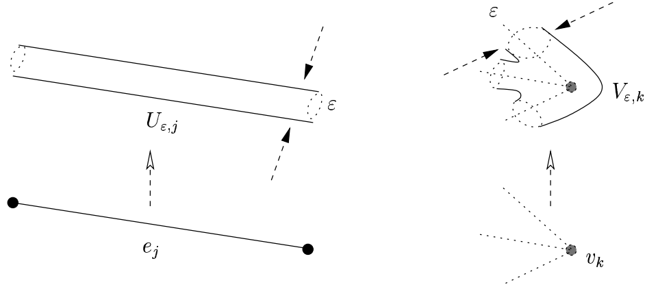
FIGURE 1. The associated edge and vertex neighbourhoods with F = \mathbb{S}^1 , i.e., U_{\varepsilon,j} and V_{\varepsilon,k} are 2-dimensional manifolds with boundary.
