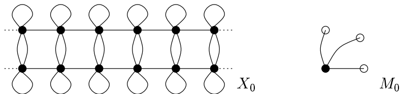
FIGURE 7. The Cayley graph associated to the group \Gamma = \mathbb{Z} \times \mathbb{Z}_2 \times \mathbb{Z}_1 , where the trivial group \mathbb{Z}_1 leads to the attachment of a loop at each vertex. On the right, the corresponding period cell is shown. Note that \Delta_{X_0} has spectral gaps in contrast to the example without loops.
