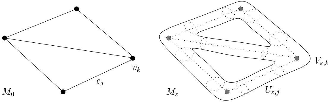
FIGURE 2. On the left, we have the graph M_0 , on the right, the associated graph-like manifold (in this case, F = \mathbb{S}^1 and M_\varepsilon is a 2-dimensional manifold).
