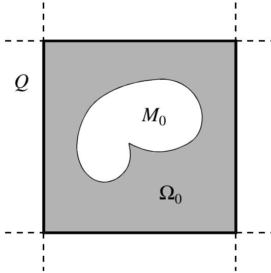
FIGURE 1. The fundamental period cell Q and the set M_0 = Q \cap M .
