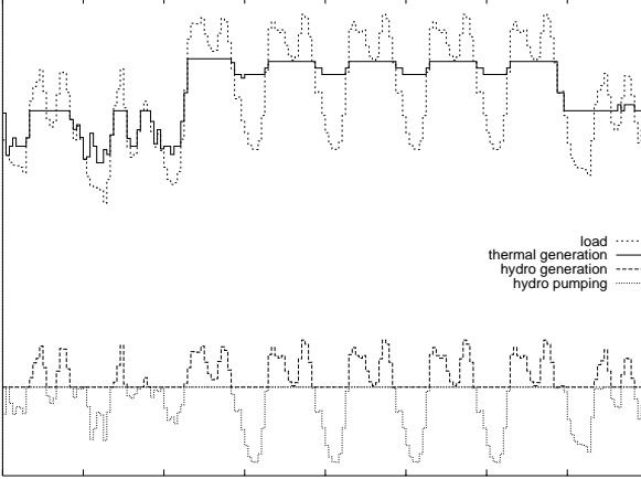
Figure 1: Load and hydro-thermal schedule
