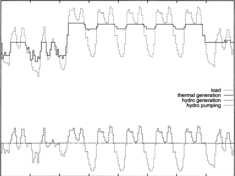
Fig. 1: load curve and hydro-thermal schedule
