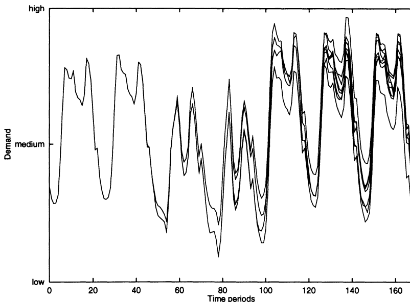
Fig. 3: Sampled load scenarios
