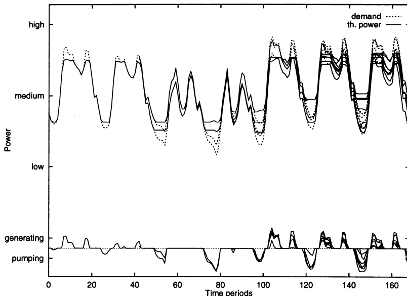
Fig. 4: Solution for the load given in Figure 3
