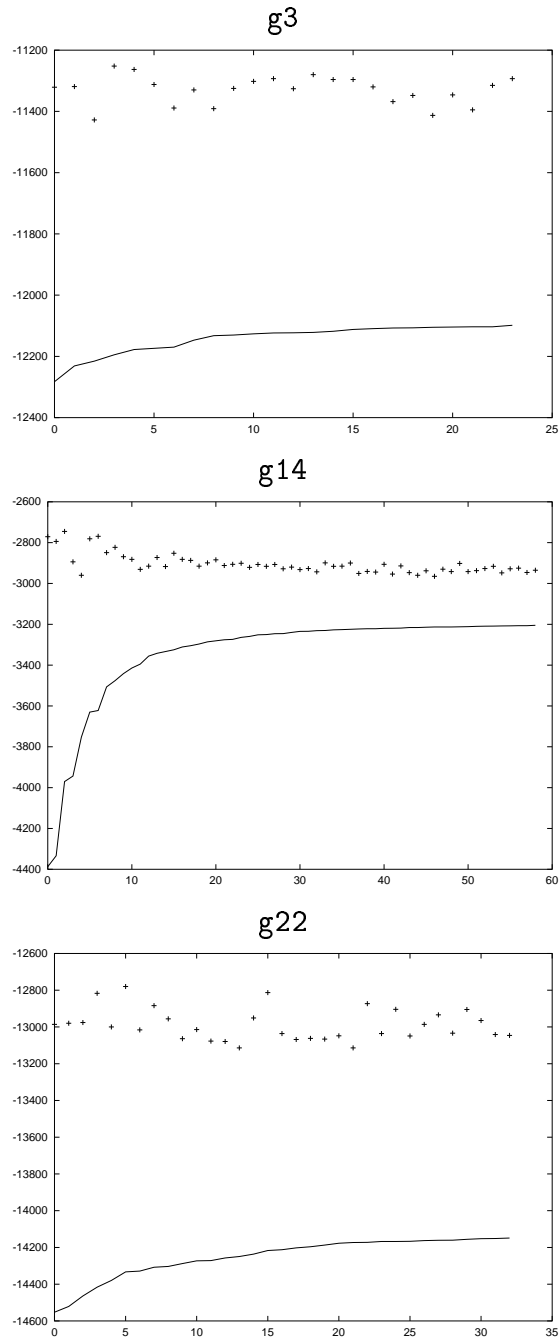
Figure 2: Plots of sequence of the values of dual points and their correspondent primal heuristic solution produced by Algorithm pathfollowing from rudy graphs g3, g14, and g22.
