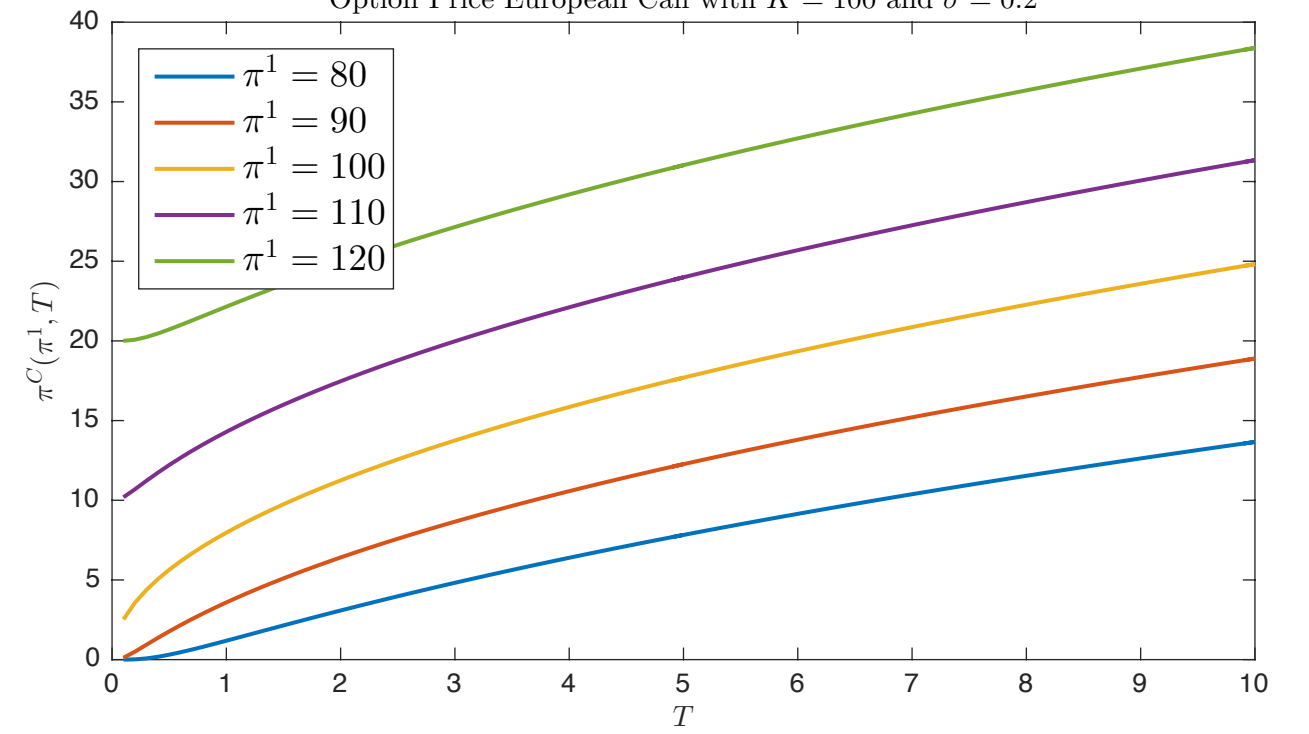
Option Price European Call with K = 100 and \sigma = 0.2
