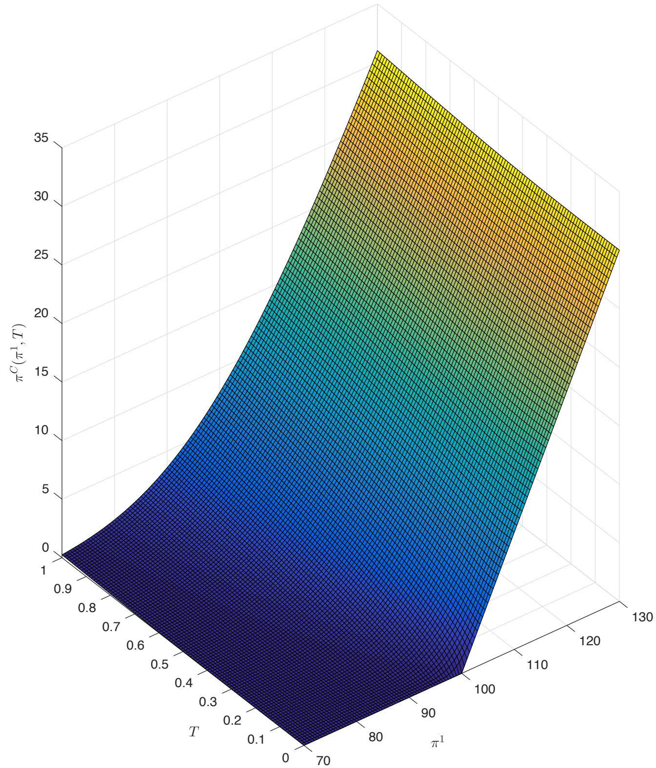
Option Price European Call with K = 100 and \sigma = 0.2
