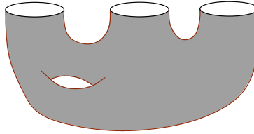
FIGURE 7. The surface \Sigma_{1,3} as in Exercise 14.12.
