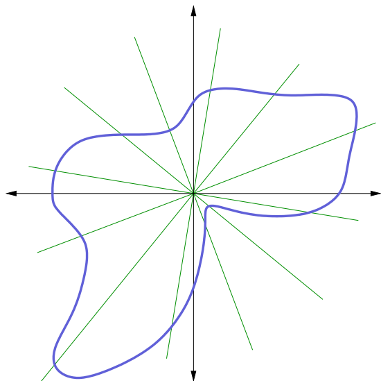
FIGURE 2. A star-shaped hypersurface in \mathbb{R}^2 .
