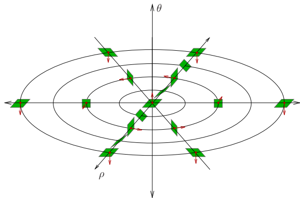
FIGURE 4. An overtwisted contact structure.
